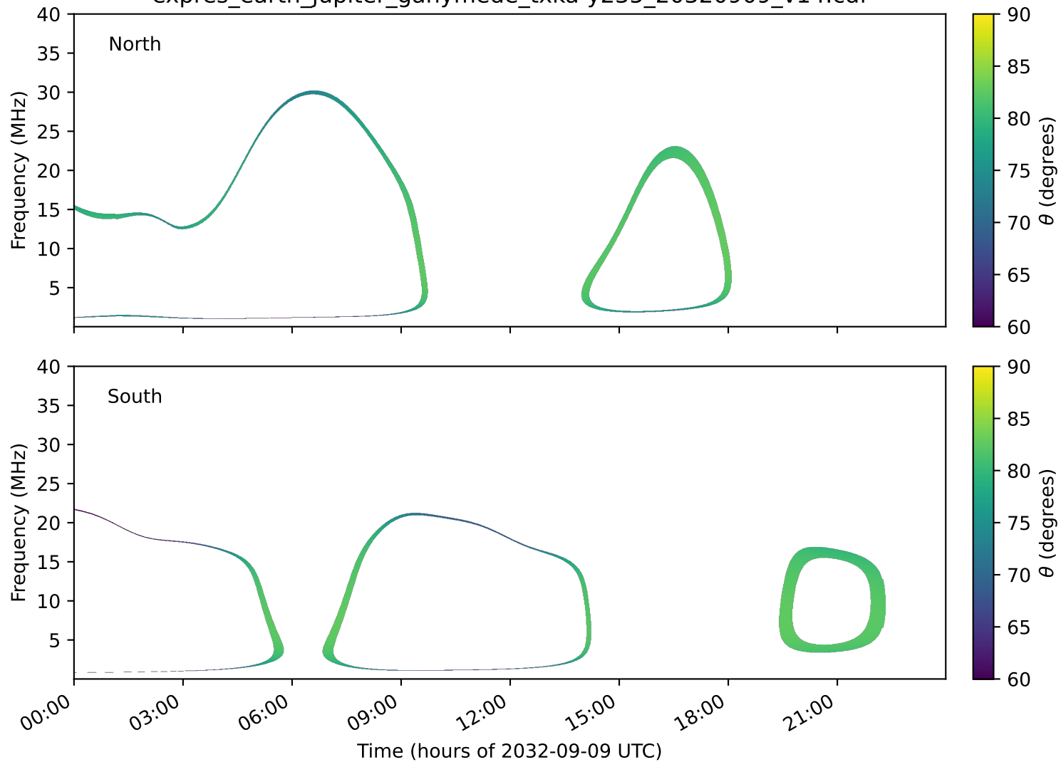
expres_earth_jupiter_ganymede_txka-y235_20320909_v14.cdf
