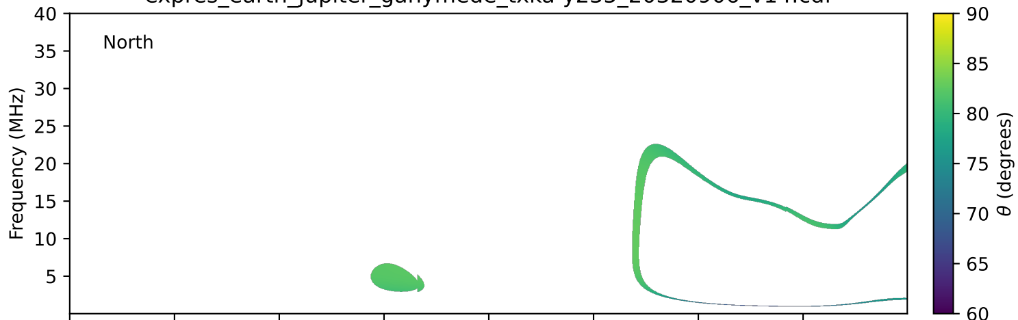
expres_earth_jupiter_ganymede_txka-y235_20320906_v14.cdf
