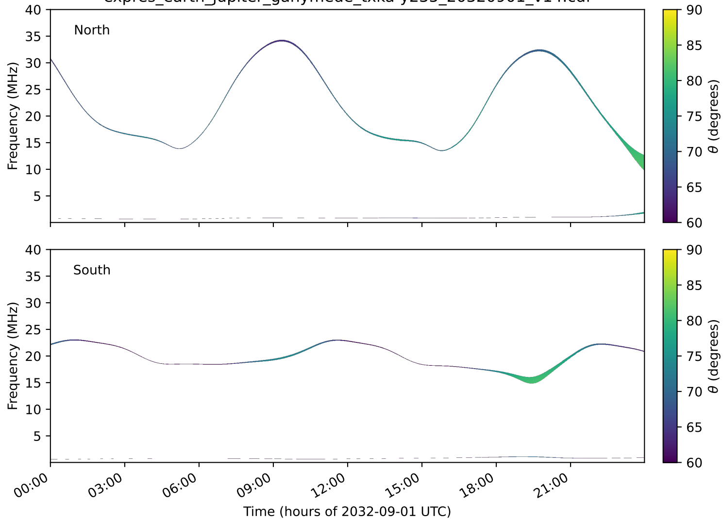
expres_earth_jupiter_ganymede_txka-y235_20320901_v14.cdf
