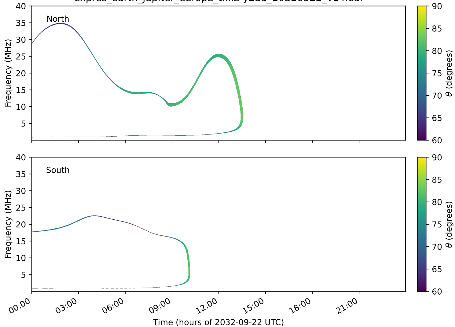
expres_earth_jupiter_europa_txka-y235_20320922_v14.cdf
