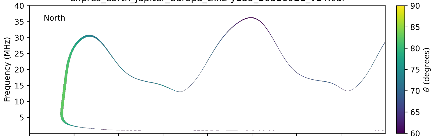
expres_earth_jupiter_europa_txka-y235_20320921_v14.cdf
