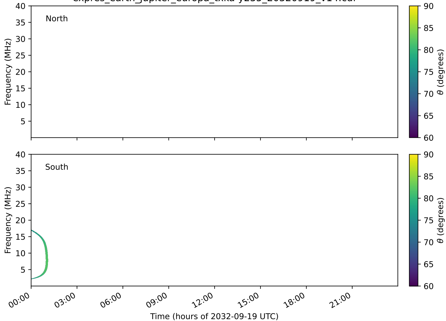
expres_earth_jupiter_europa_txka-y235_20320919_v14.cdf
