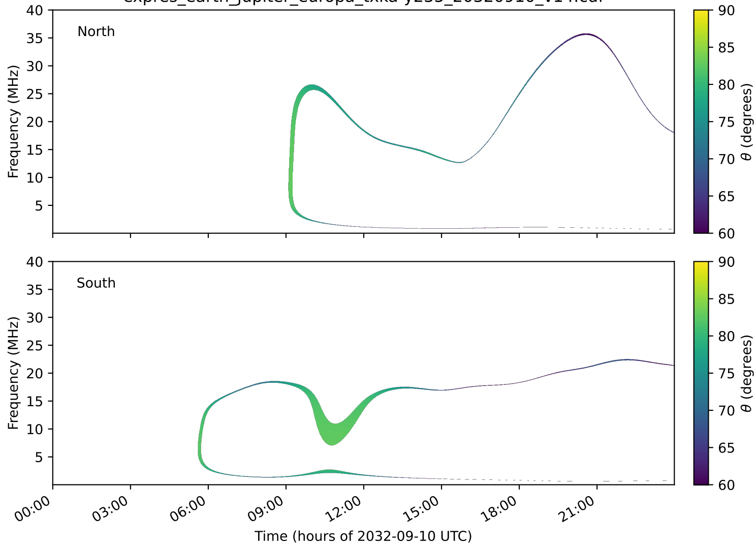
expres_earth_jupiter_europa_txka-y235_20320910_v14.cdf
