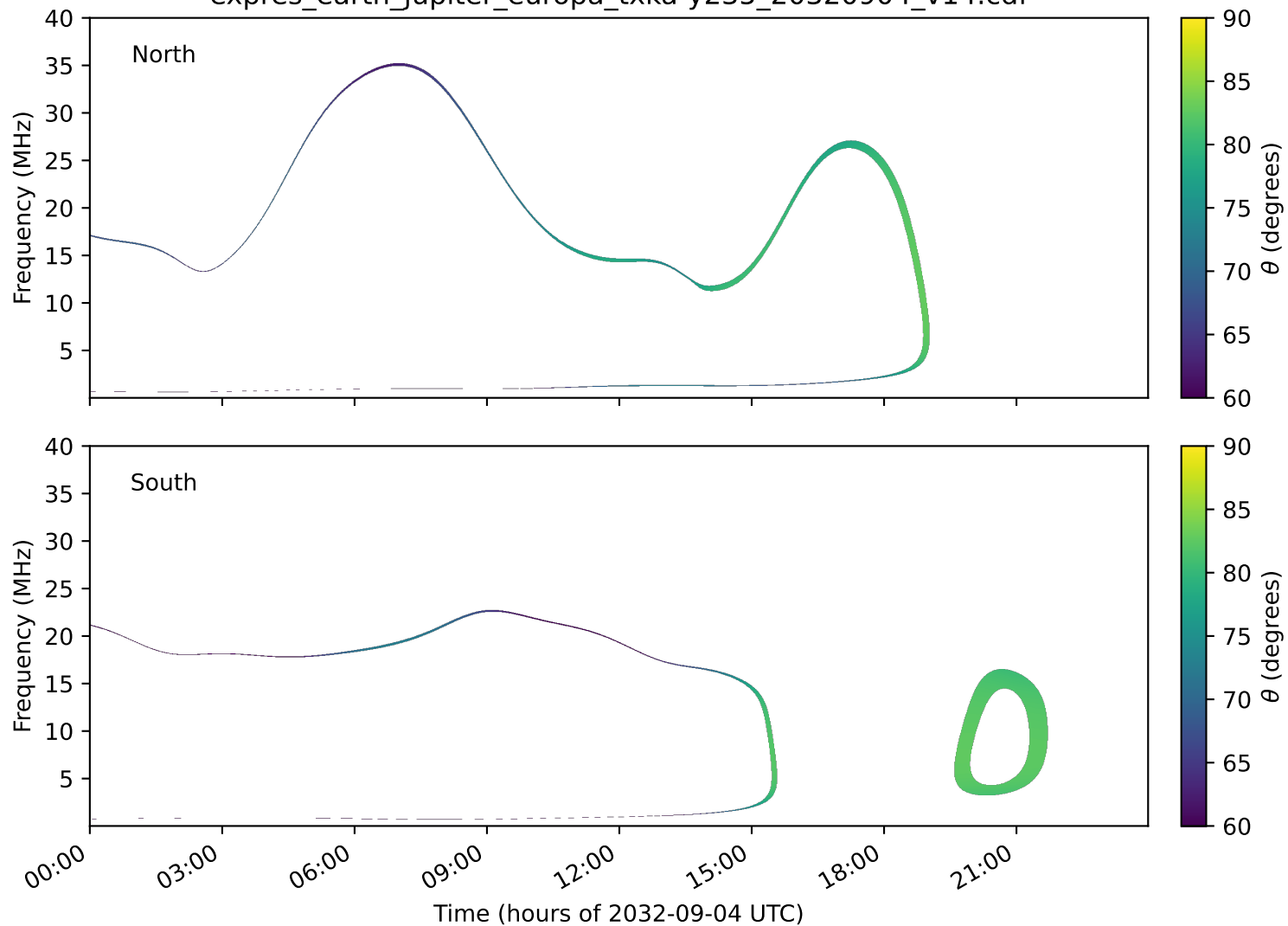
expres_earth_jupiter_europa_txka-y235_20320904_v14.cdf
