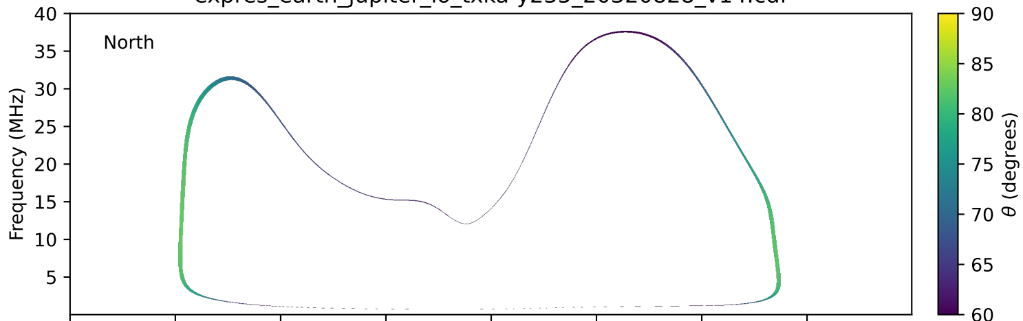
expres_earth_jupiter_io_txka-y235_20320828_v14.cdf
