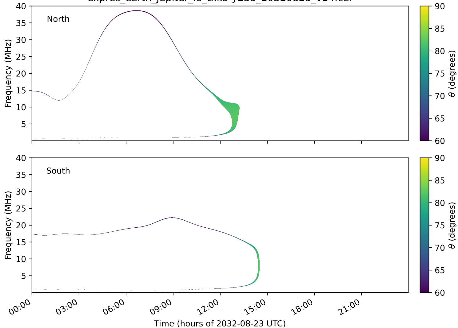
expres_earth_jupiter_io_txka-y235_20320823_v14.cdf
