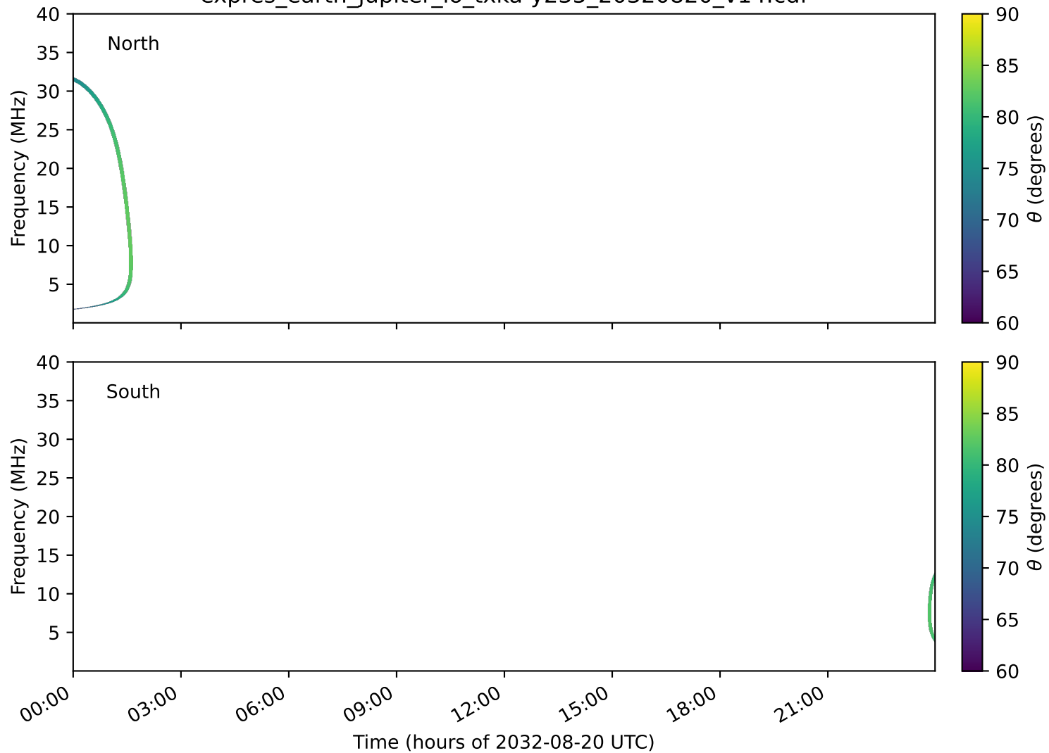
expres_earth_jupiter_io_txka-y235_20320820_v14.cdf
