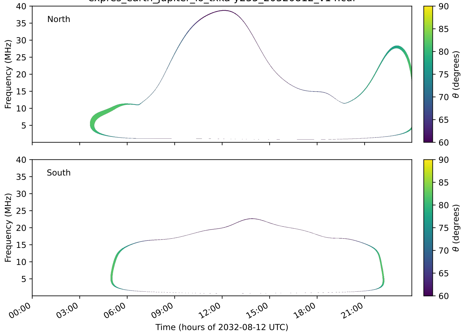
expres_earth_jupiter_io_txka-y235_20320812_v14.cdf
