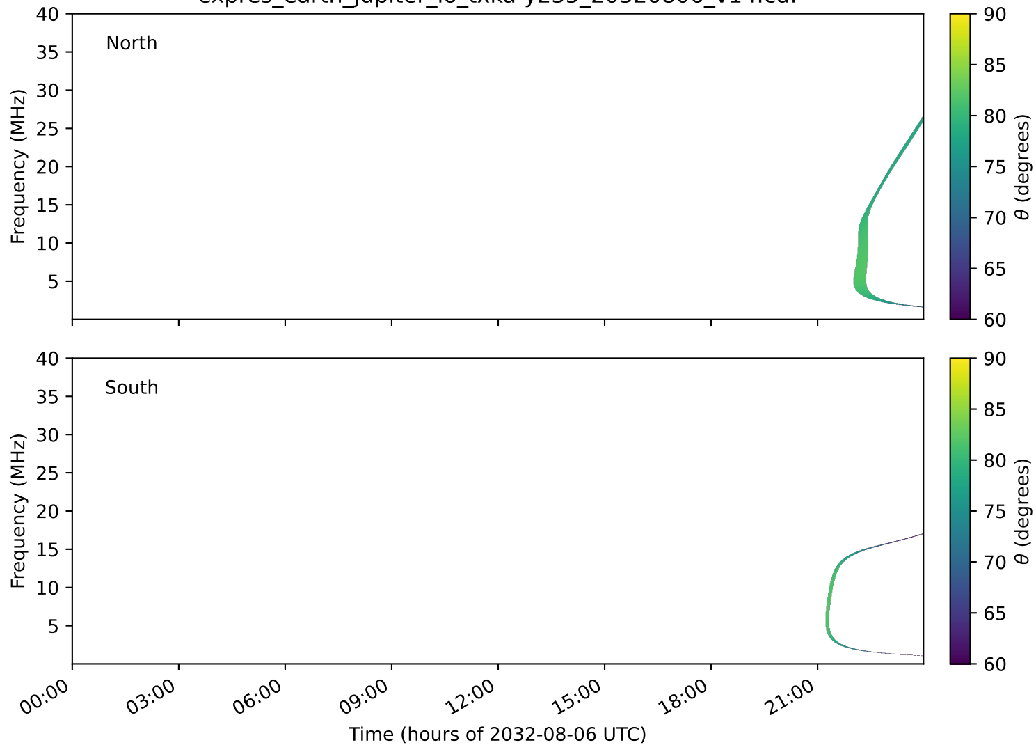
expres_earth_jupiter_io_txka-y235_20320806_v14.cdf
