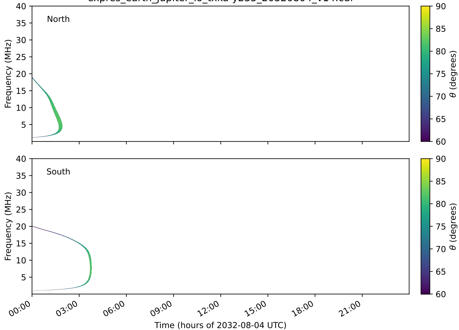
expres_earth_jupiter_io_txka-y235_20320804_v14.cdf
