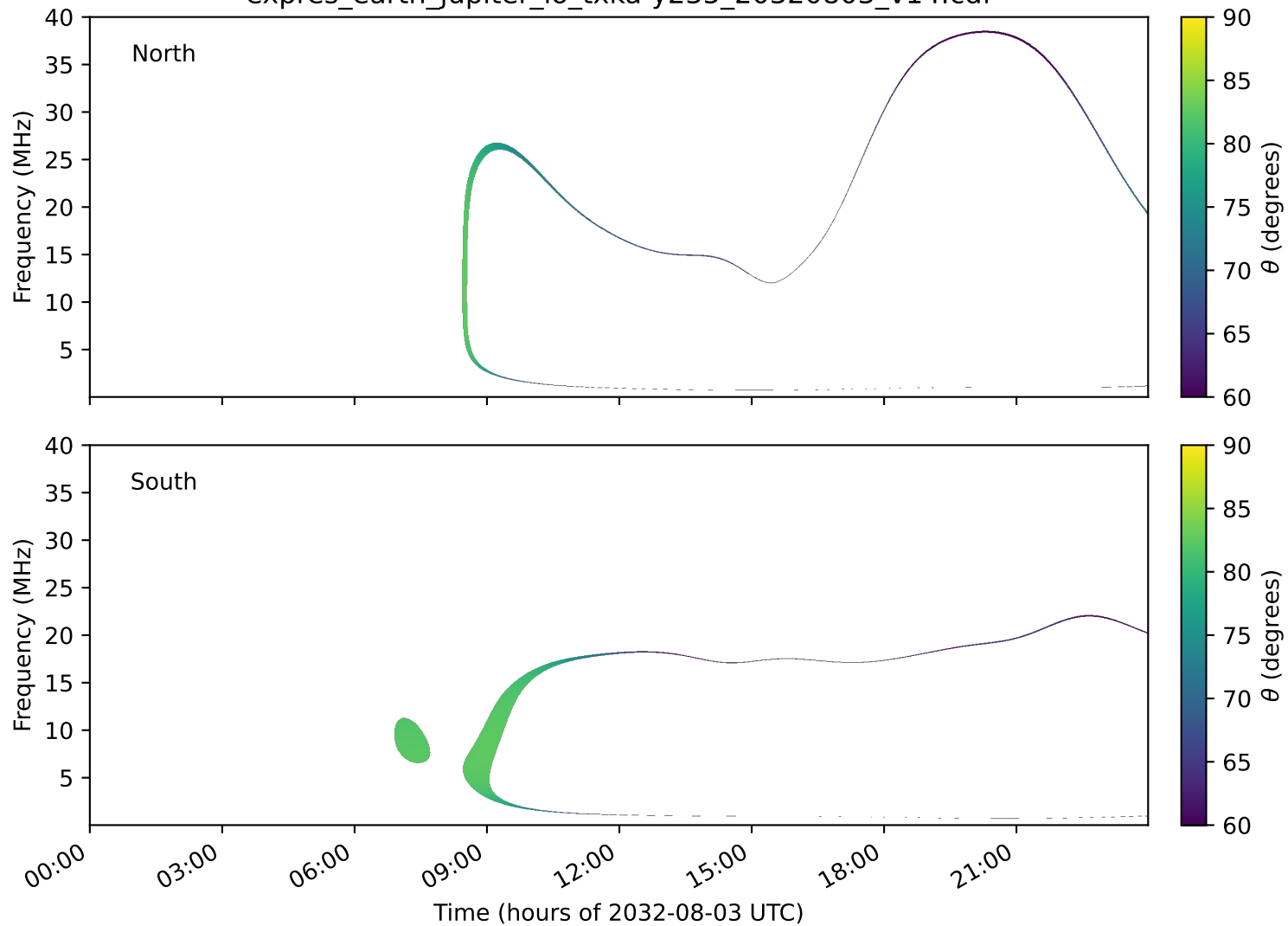
expres_earth_jupiter_io_txka-y235_20320803_v14.cdf
