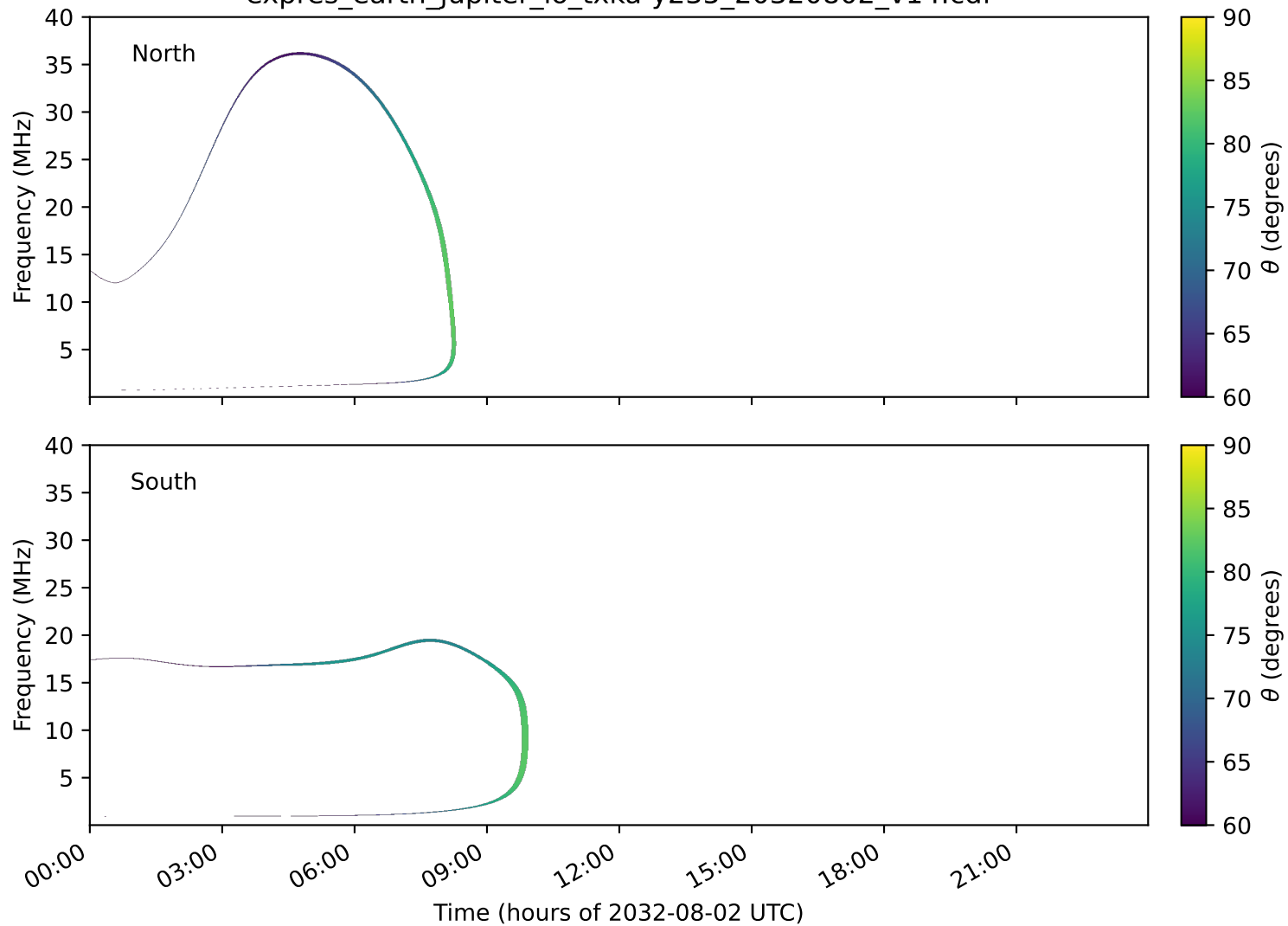
expres_earth_jupiter_io_txka-y235_20320802_v14.cdf
