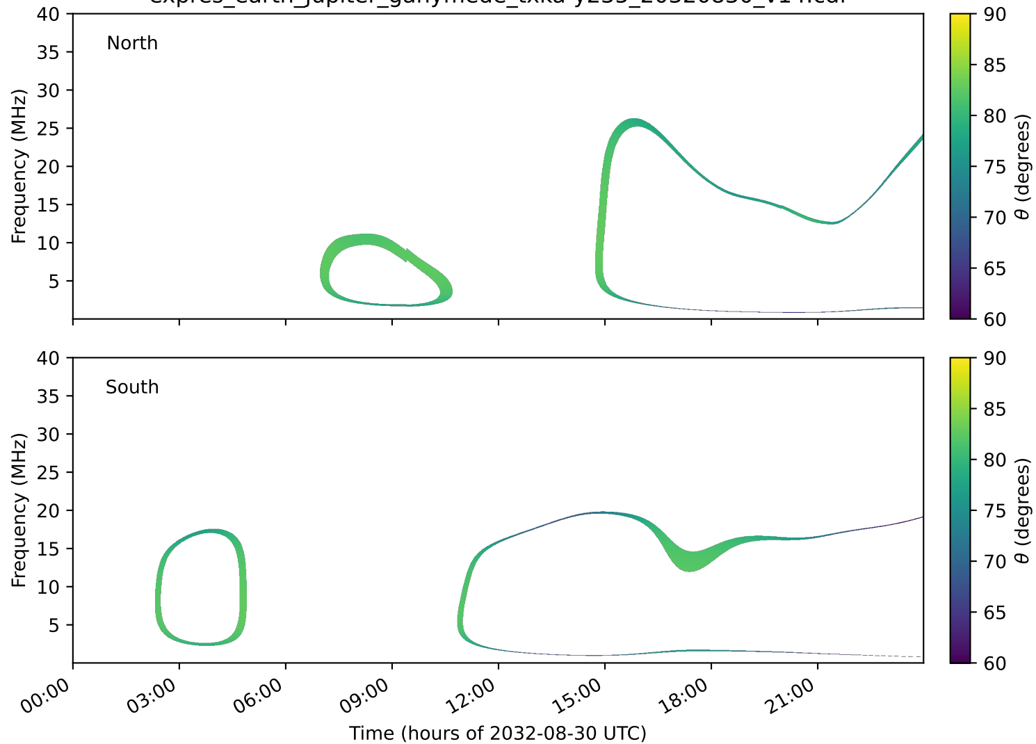
expres_earth_jupiter_ganymede_txka-y235_20320830_v14.cdf
