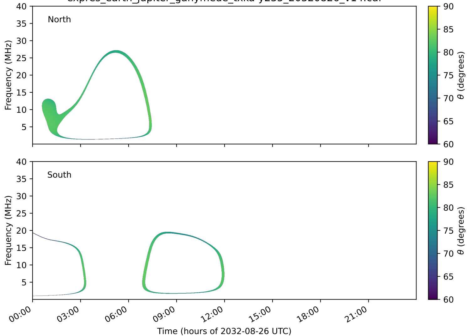
expres_earth_jupiter_ganymede_txka-y235_20320826_v14.cdf
