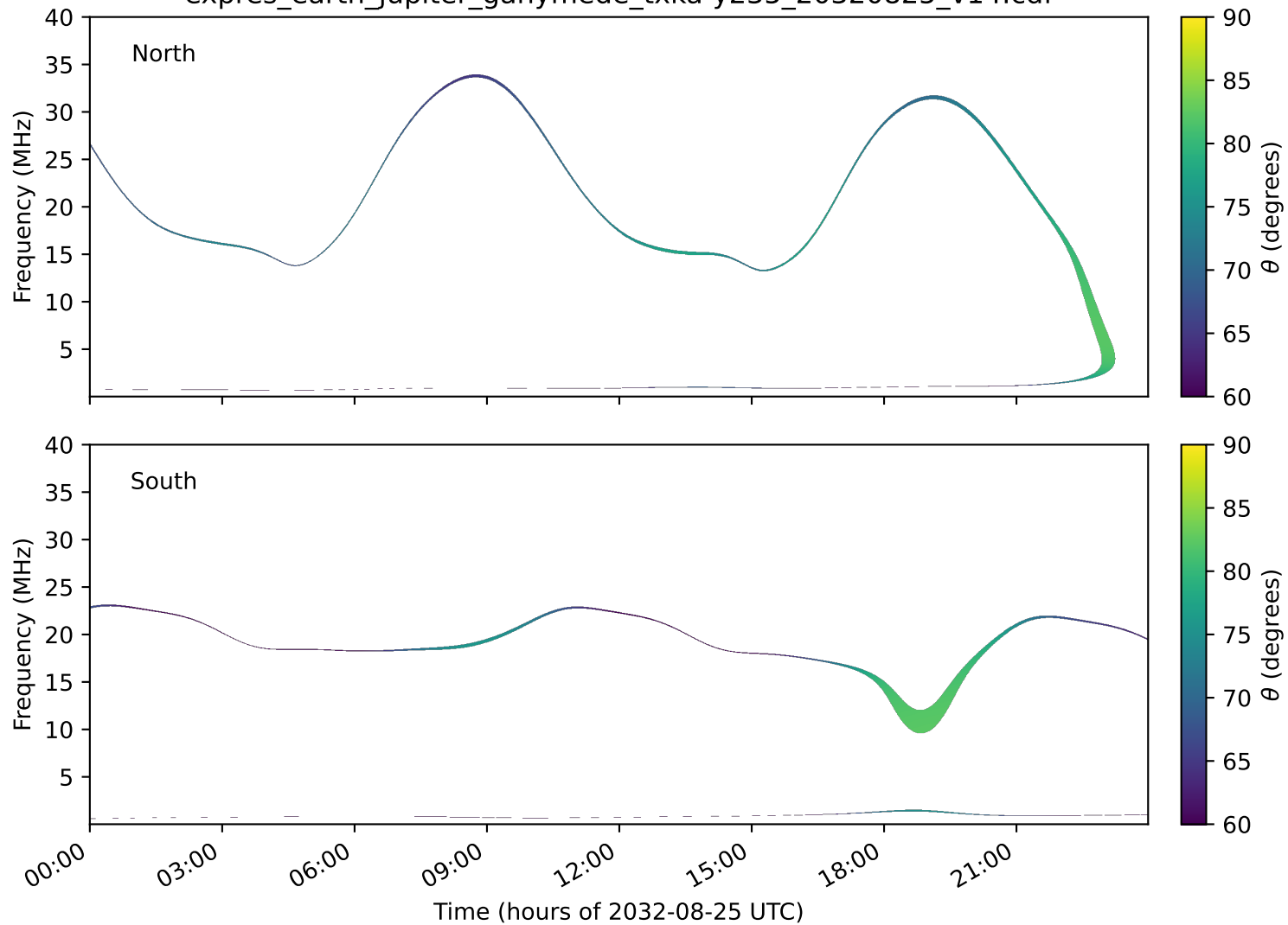
expres_earth_jupiter_ganymede_txka-y235_20320825_v14.cdf
