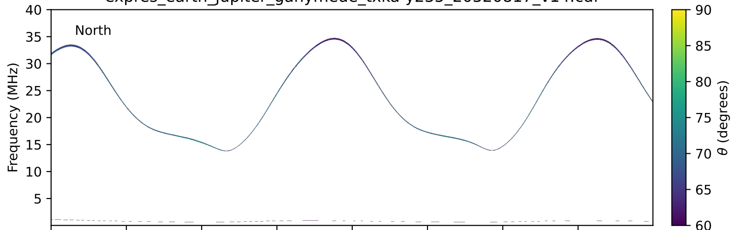
expres_earth_jupiter_ganymede_txka-y235_20320817_v14.cdf
