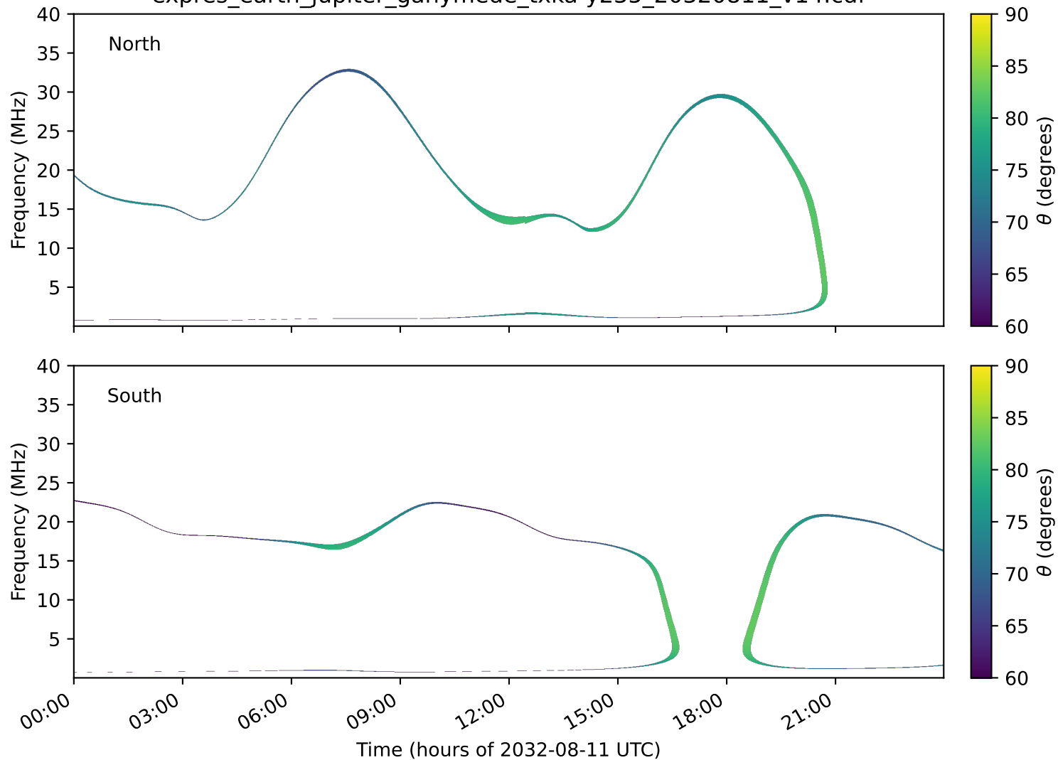
expres_earth_jupiter_ganymede_txka-y235_20320811_v14.cdf
