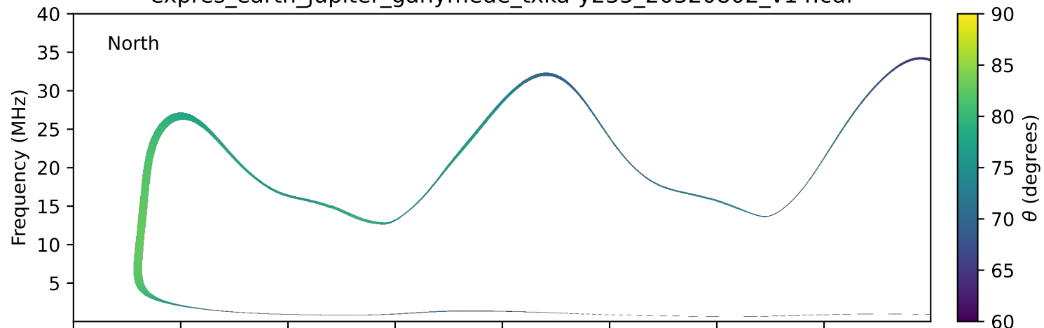
expres_earth_jupiter_ganymede_txka-y235_20320802_v14.cdf
