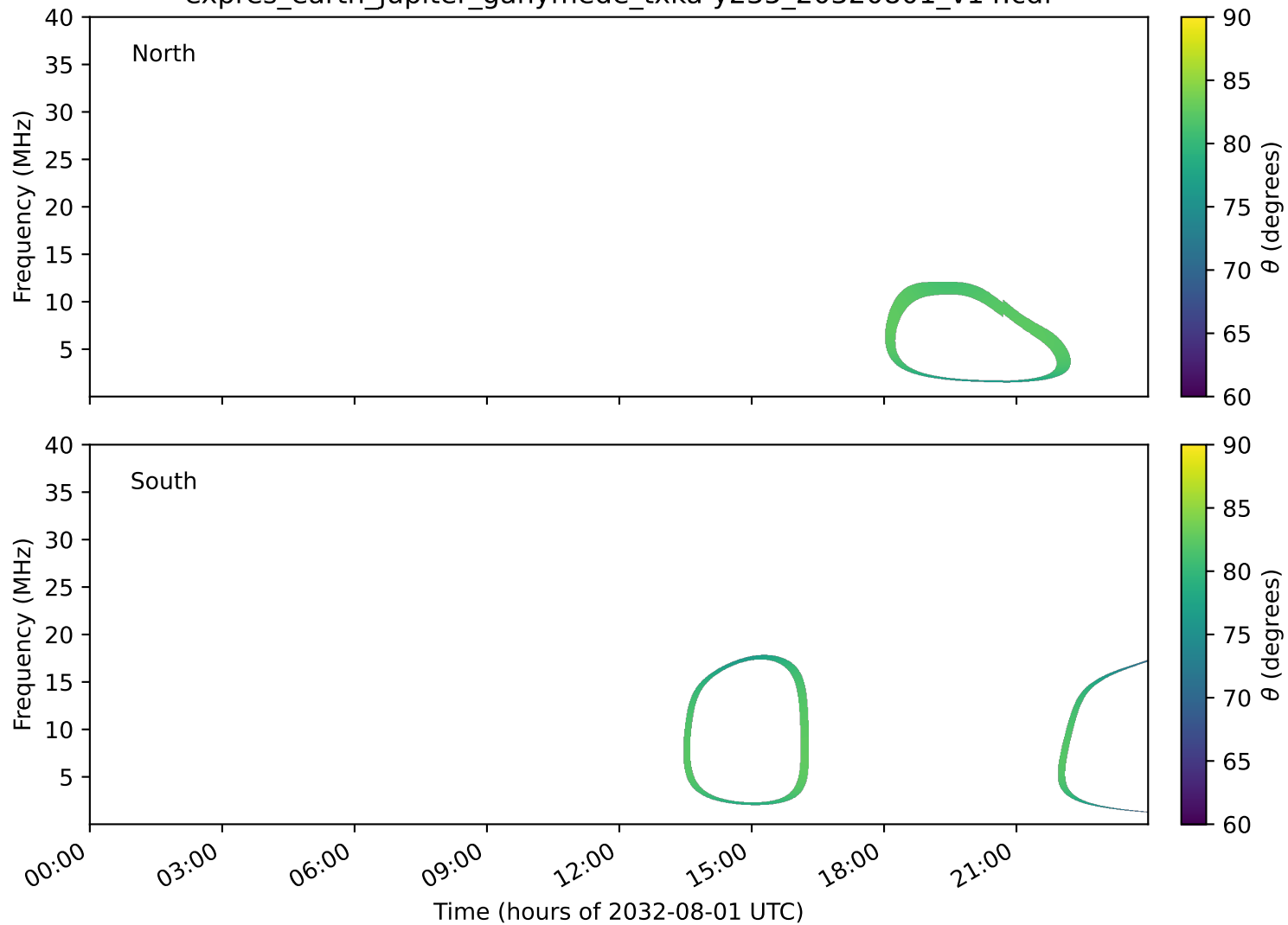
expres_earth_jupiter_ganymede_txka-y235_20320801_v14.cdf
