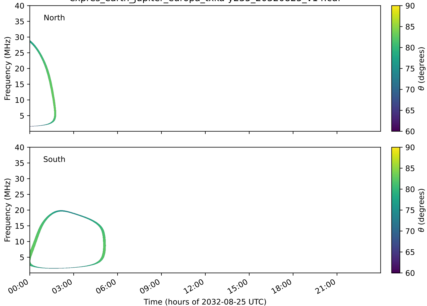
expres_earth_jupiter_europa_txka-y235_20320825_v14.cdf
