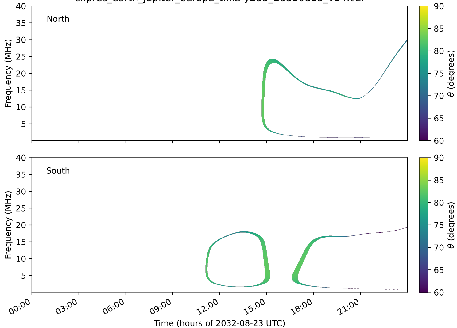
expres_earth_jupiter_europa_txka-y235_20320823_v14.cdf
