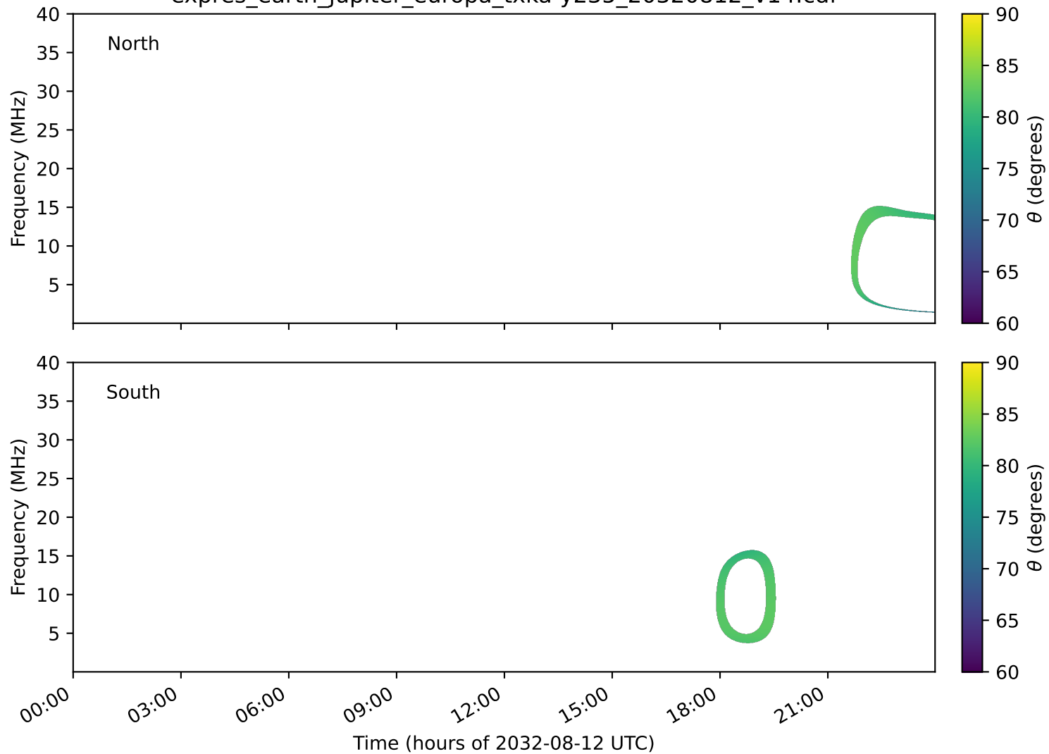
expres_earth_jupiter_europa_txka-y235_20320812_v14.cdf
