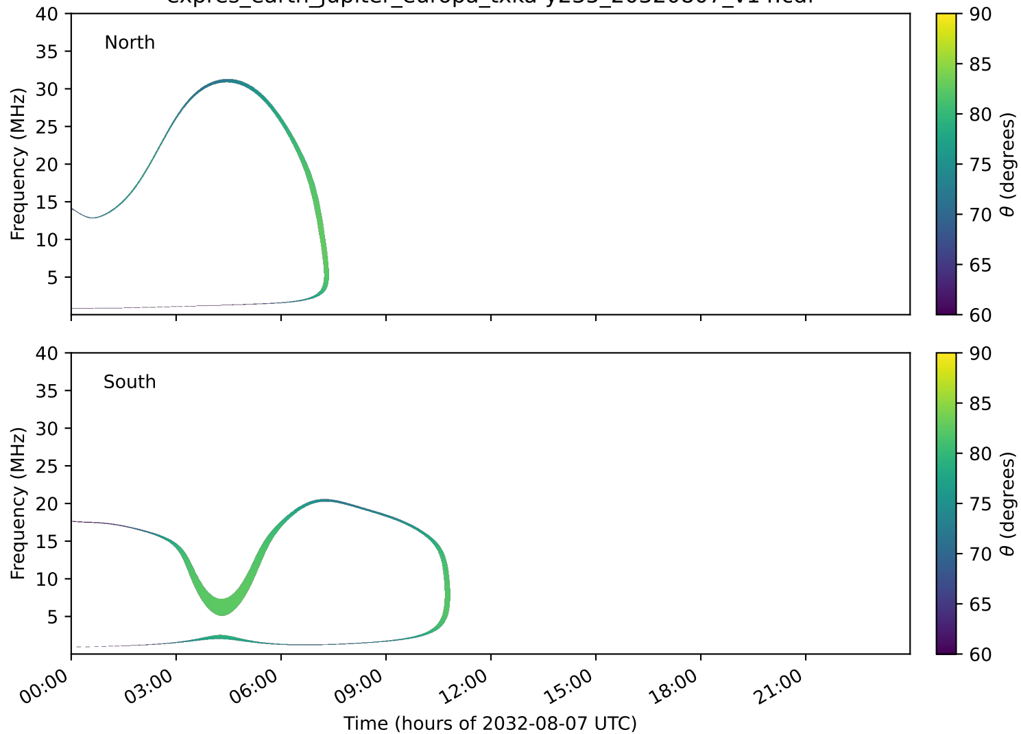
expres_earth_jupiter_europa_txka-y235_20320807_v14.cdf
