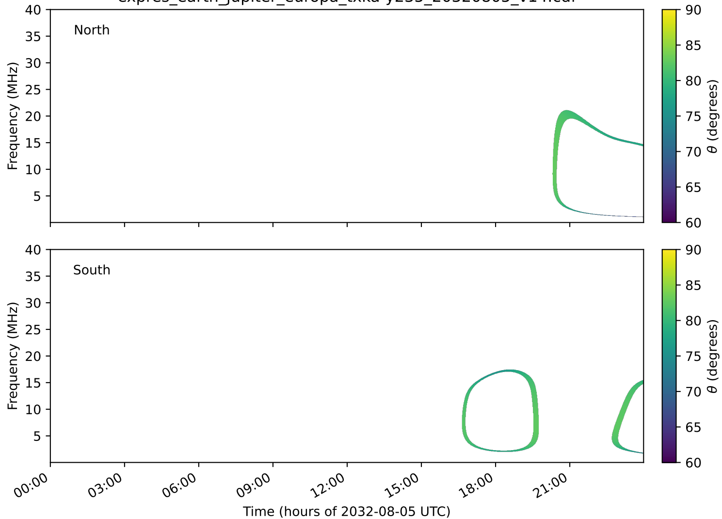
expres_earth_jupiter_europa_txka-y235_20320805_v14.cdf
