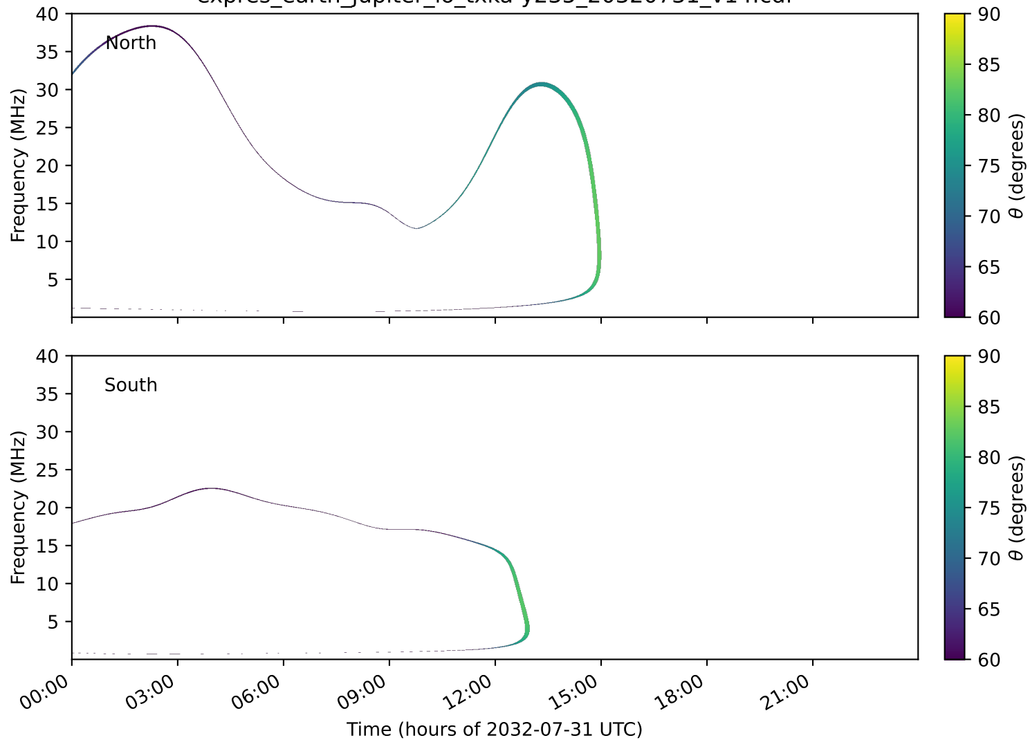
expres_earth_jupiter_io_txka-y235_20320731_v14.cdf
