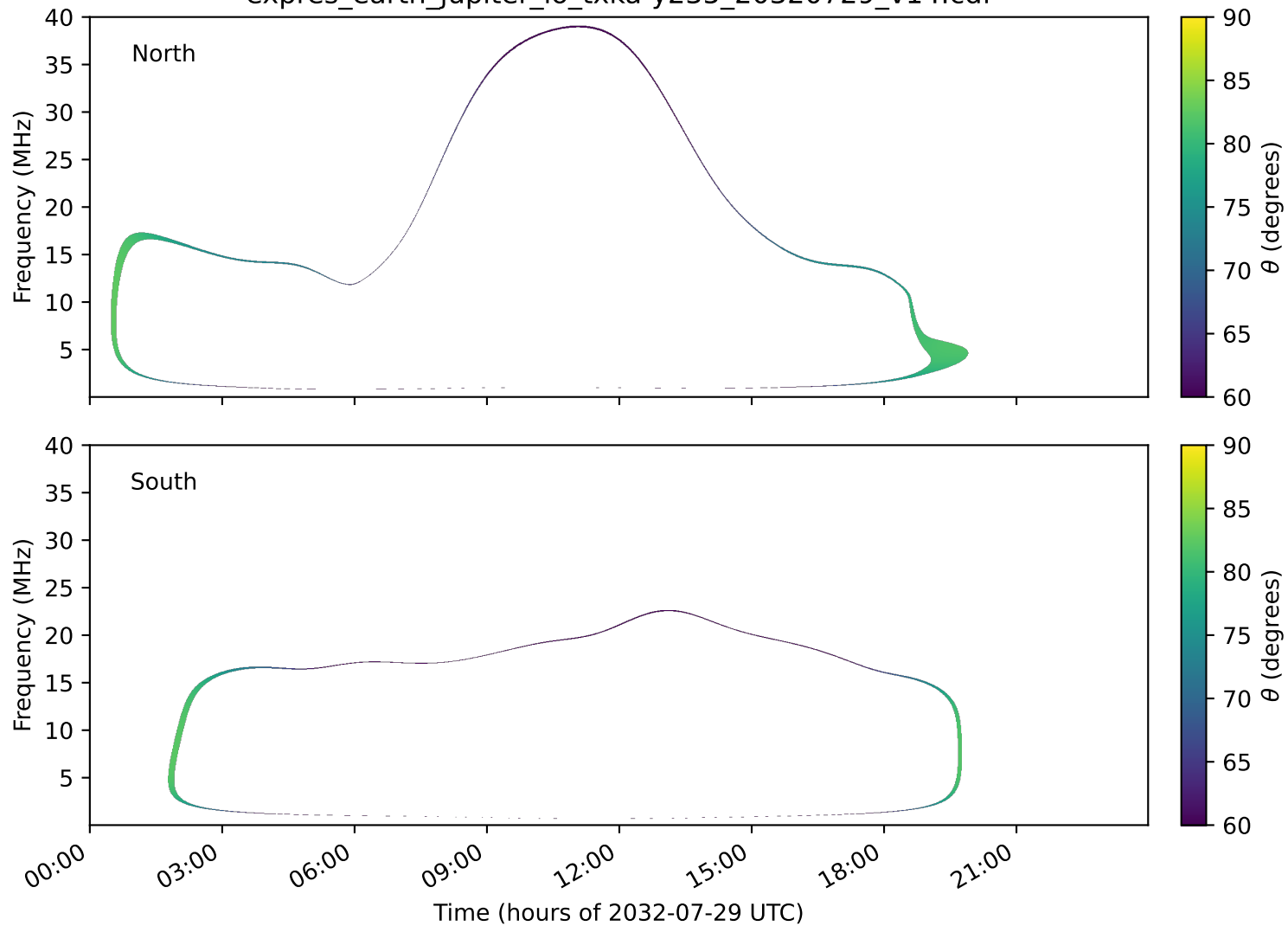
expres_earth_jupiter_io_txka-y235_20320729_v14.cdf
