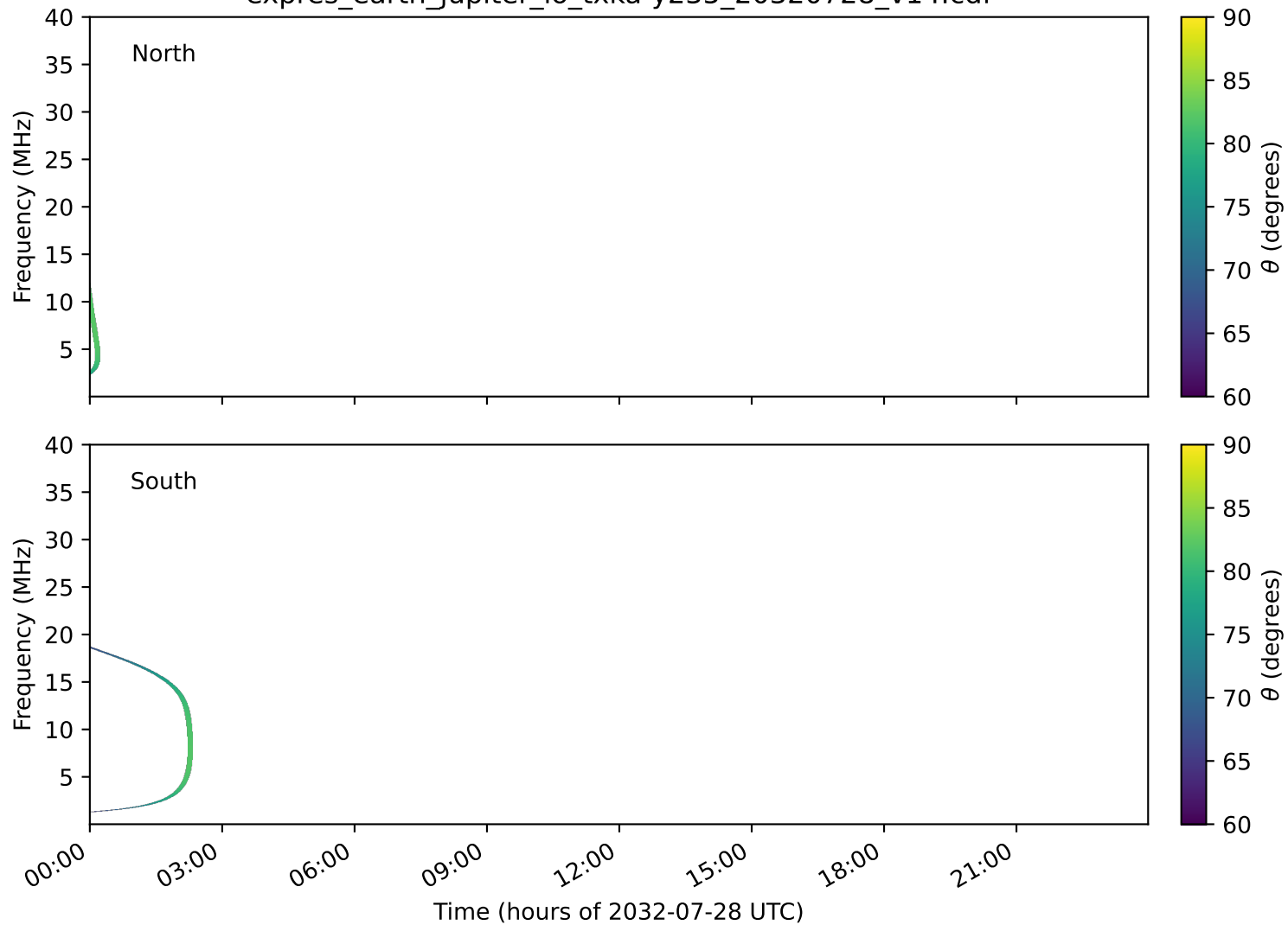
expres_earth_jupiter_io_txka-y235_20320728_v14.cdf
