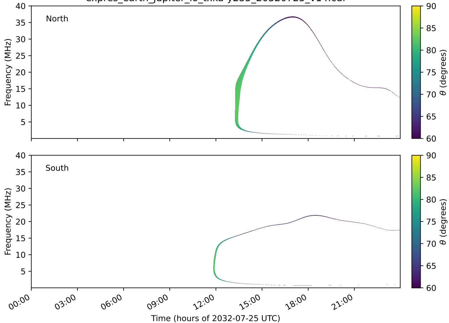
expres_earth_jupiter_io_txka-y235_20320725_v14.cdf
