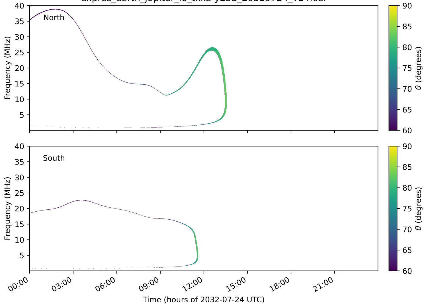
expres_earth_jupiter_io_txka-y235_20320724_v14.cdf
