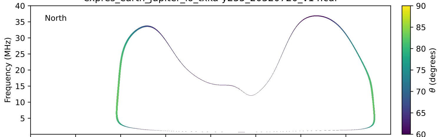
expres_earth_jupiter_io_txka-y235_20320720_v14.cdf
