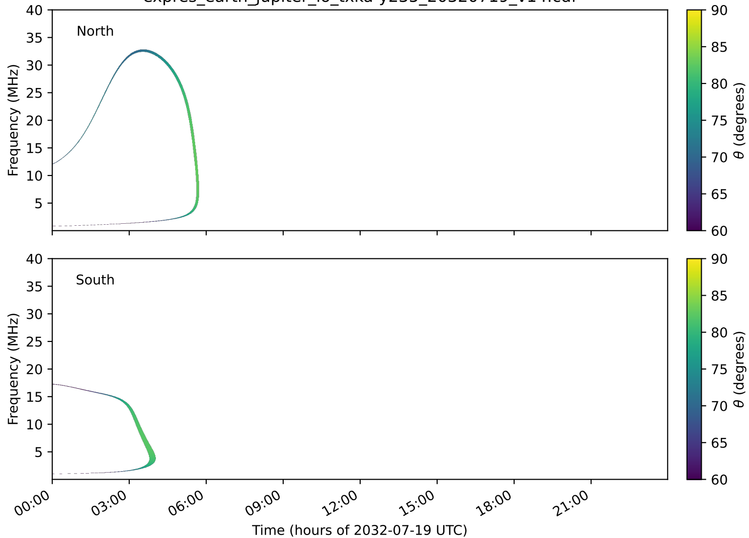
expres_earth_jupiter_io_txka-y235_20320719_v14.cdf
