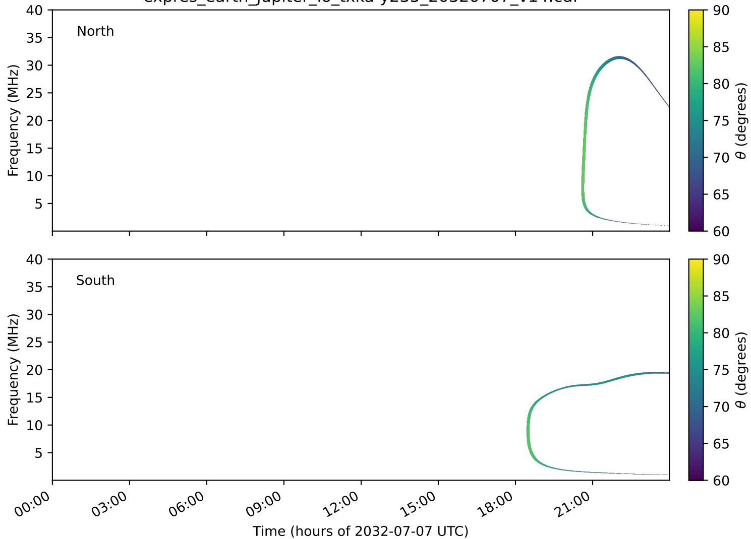
expres_earth_jupiter_io_txka-y235_20320707_v14.cdf
