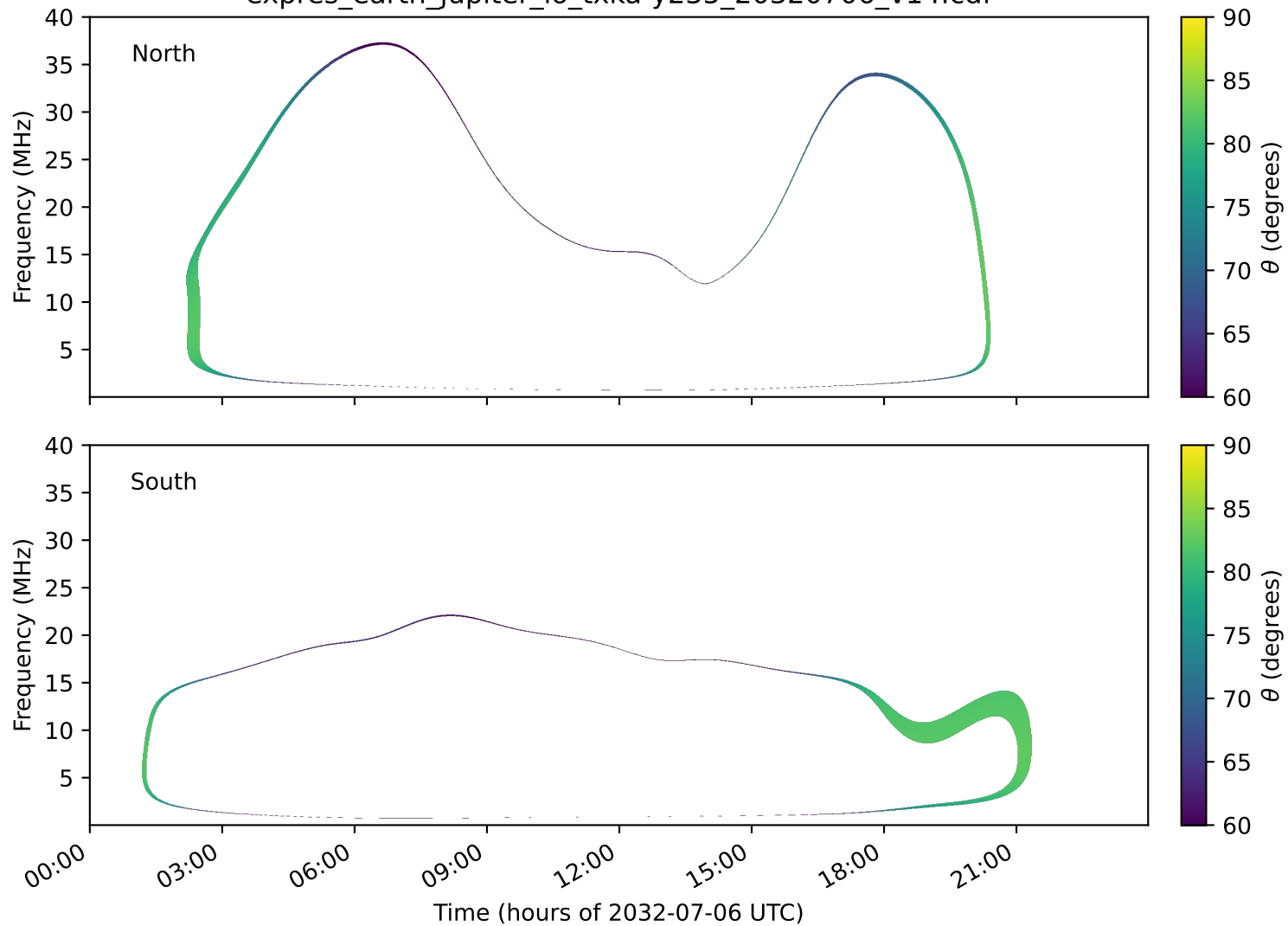
expres_earth_jupiter_io_txka-y235_20320706_v14.cdf
