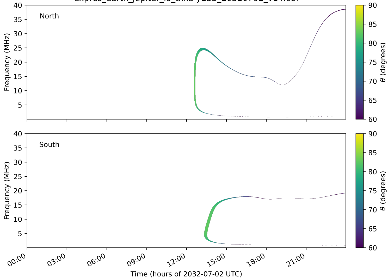
expres_earth_jupiter_io_txka-y235_20320702_v14.cdf
