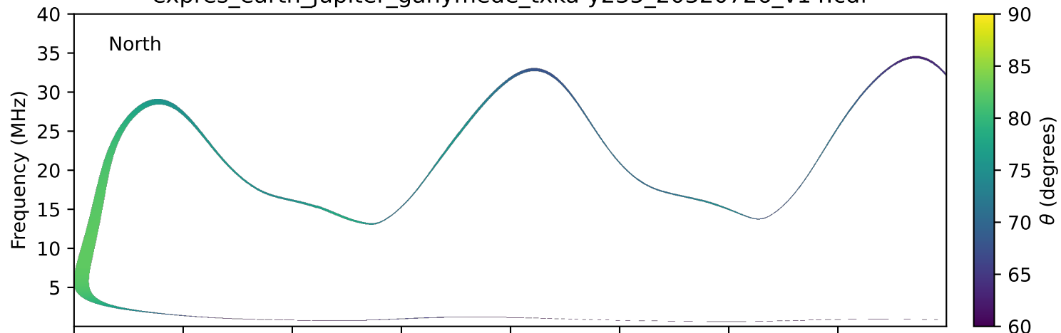
expres_earth_jupiter_ganymede_txka-y235_20320726_v14.cdf
