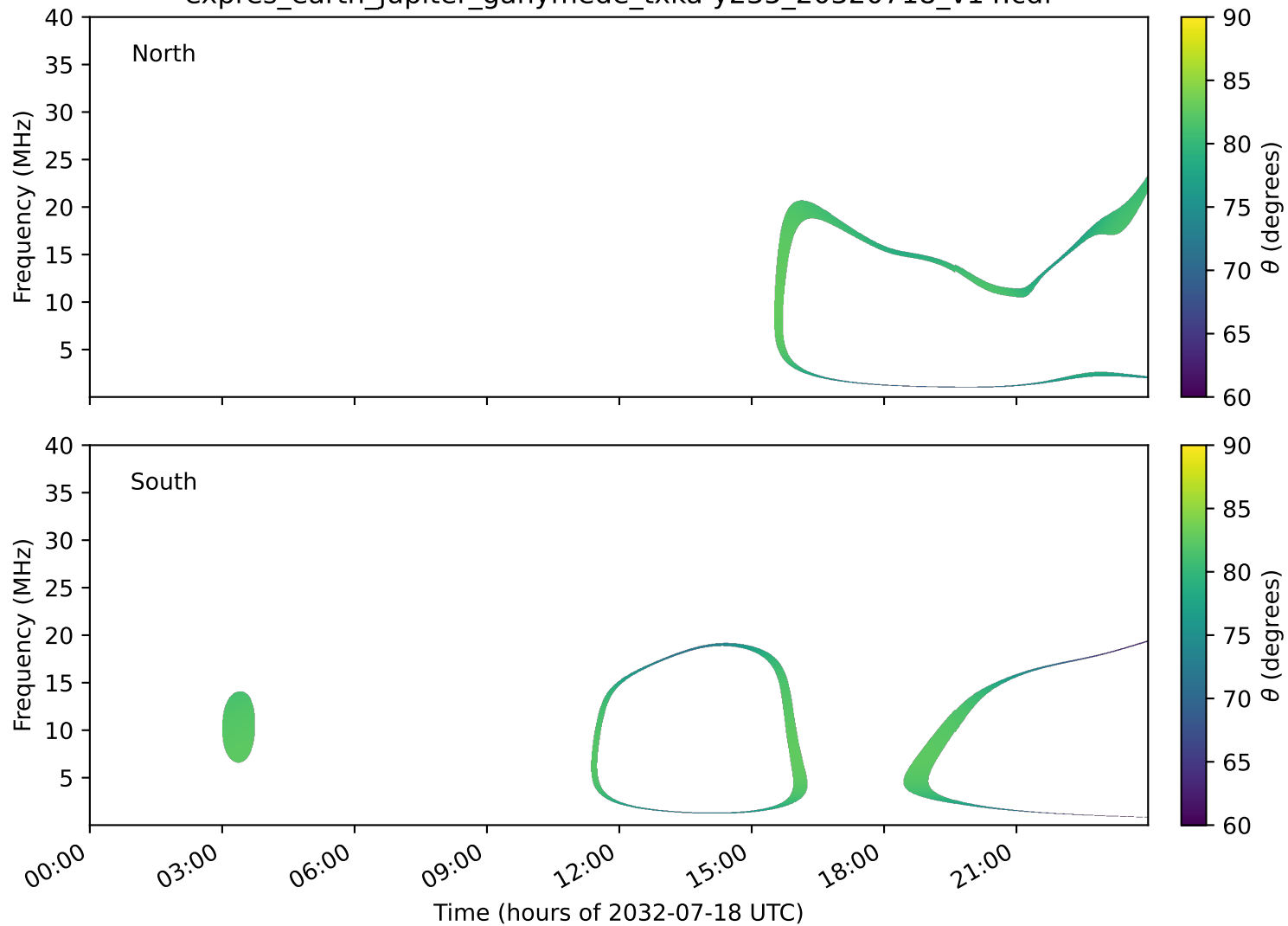
expres_earth_jupiter_ganymede_txka-y235_20320718_v14.cdf
