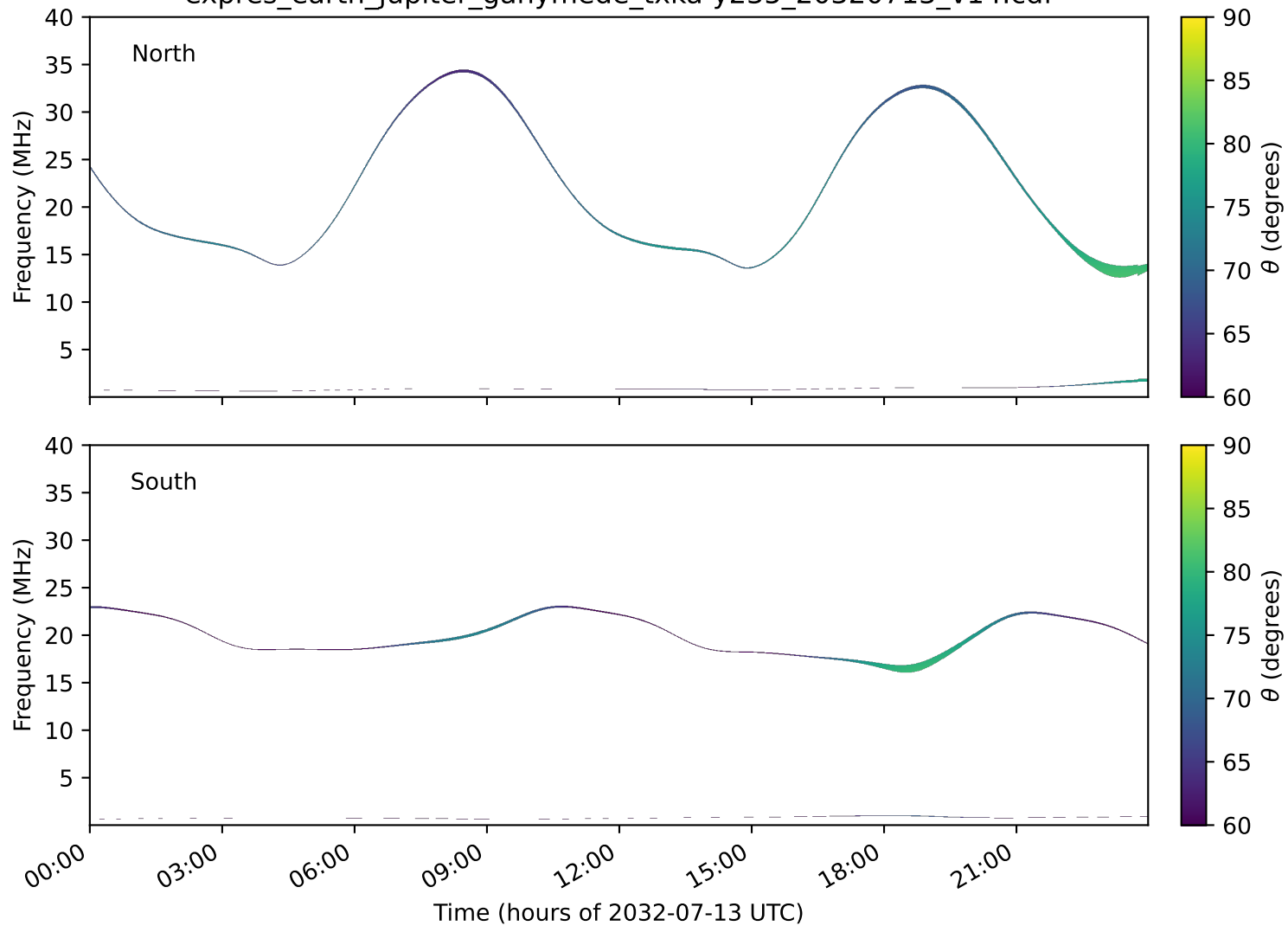
expres_earth_jupiter_ganymede_txka-y235_20320713_v14.cdf
