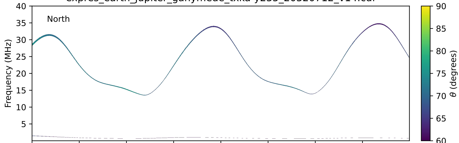
expres_earth_jupiter_ganymede_txka-y235_20320712_v14.cdf
