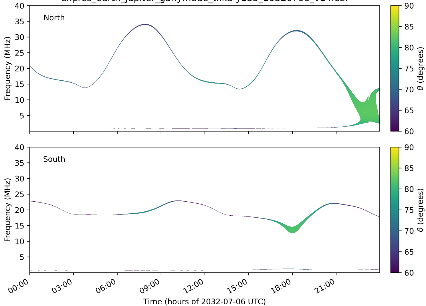
expres_earth_jupiter_ganymede_txka-y235_20320706_v14.cdf
