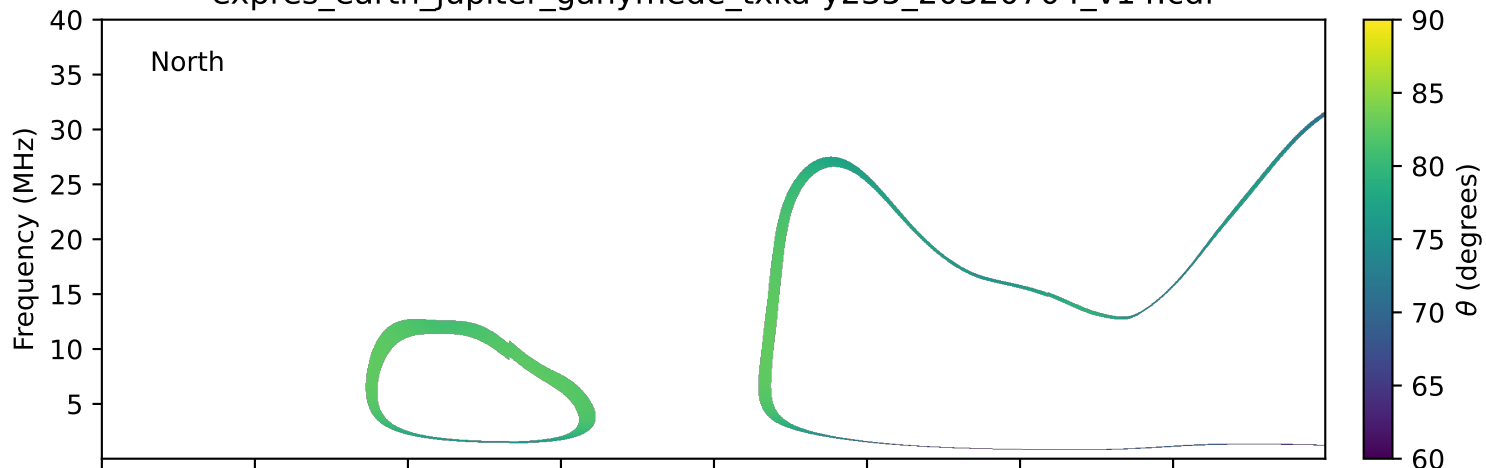
expres_earth_jupiter_ganymede_txka-y235_20320704_v14.cdf
