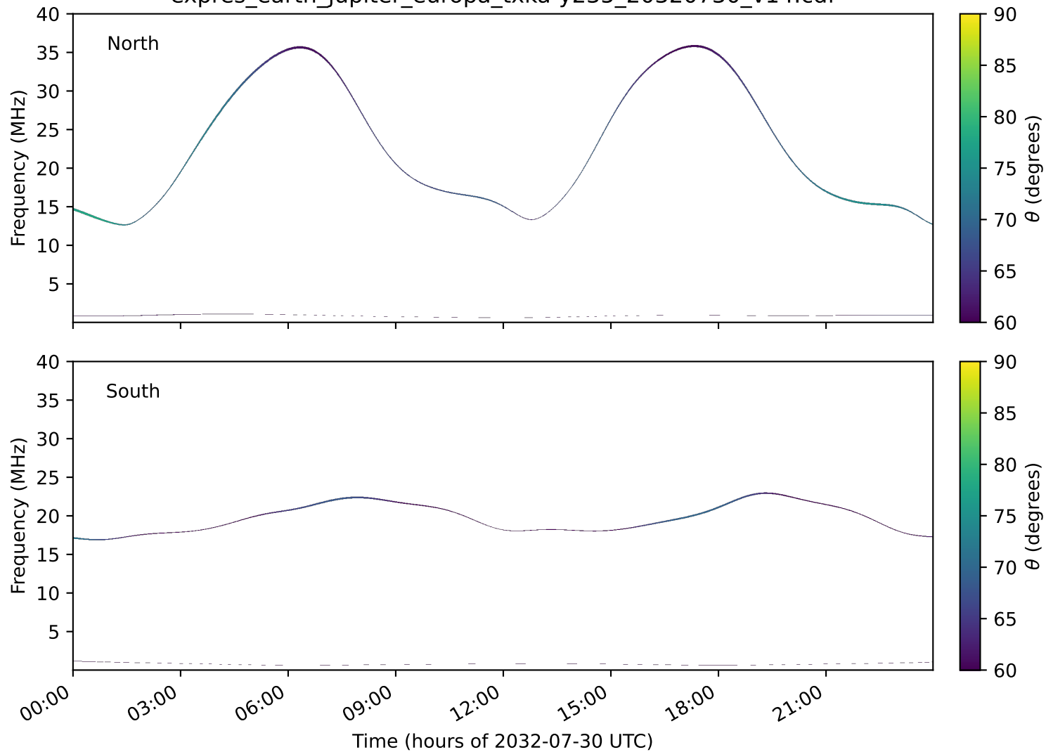
expres_earth_jupiter_europa_txka-y235_20320730_v14.cdf
