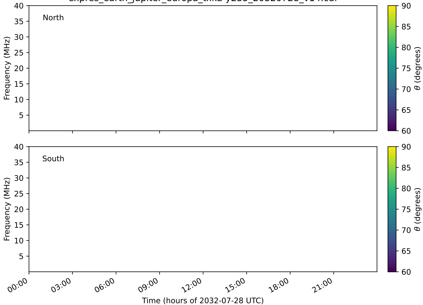
expres_earth_jupiter_europa_txka-y235_20320728_v14.cdf
