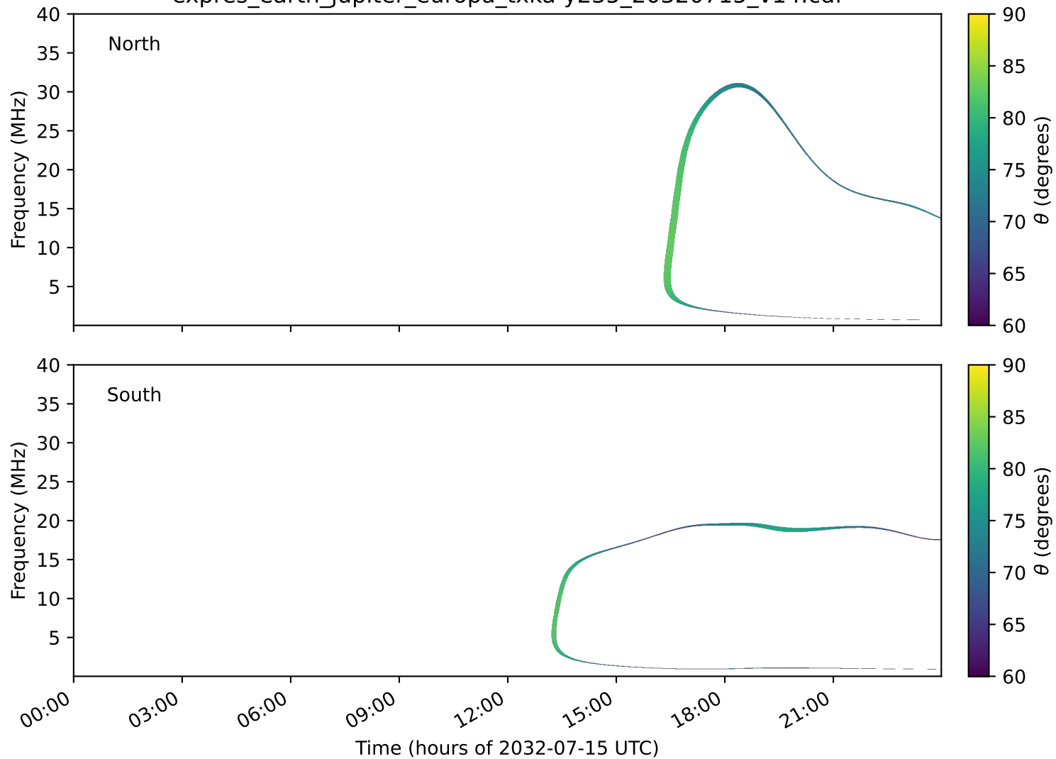
expres_earth_jupiter_europa_txka-y235_20320715_v14.cdf
