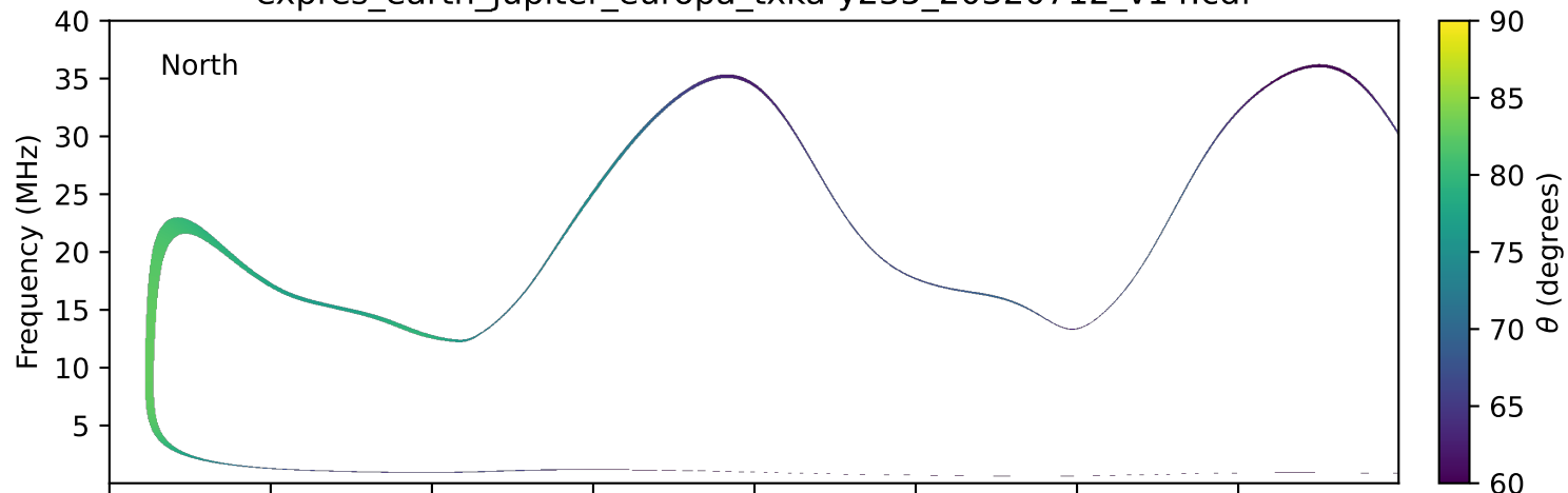
expres_earth_jupiter_europa_txka-y235_20320712_v14.cdf
