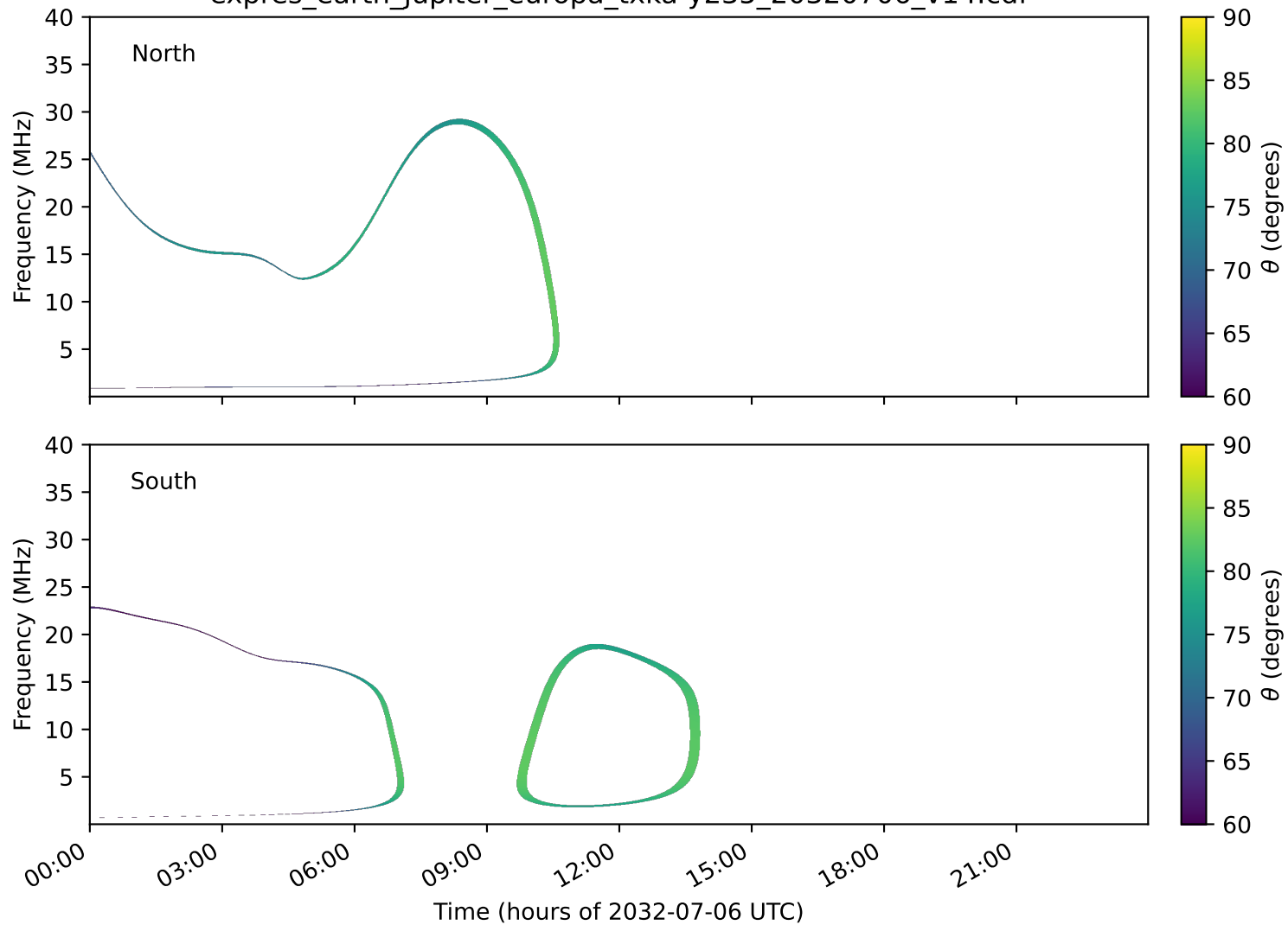
expres_earth_jupiter_europa_txka-y235_20320706_v14.cdf
