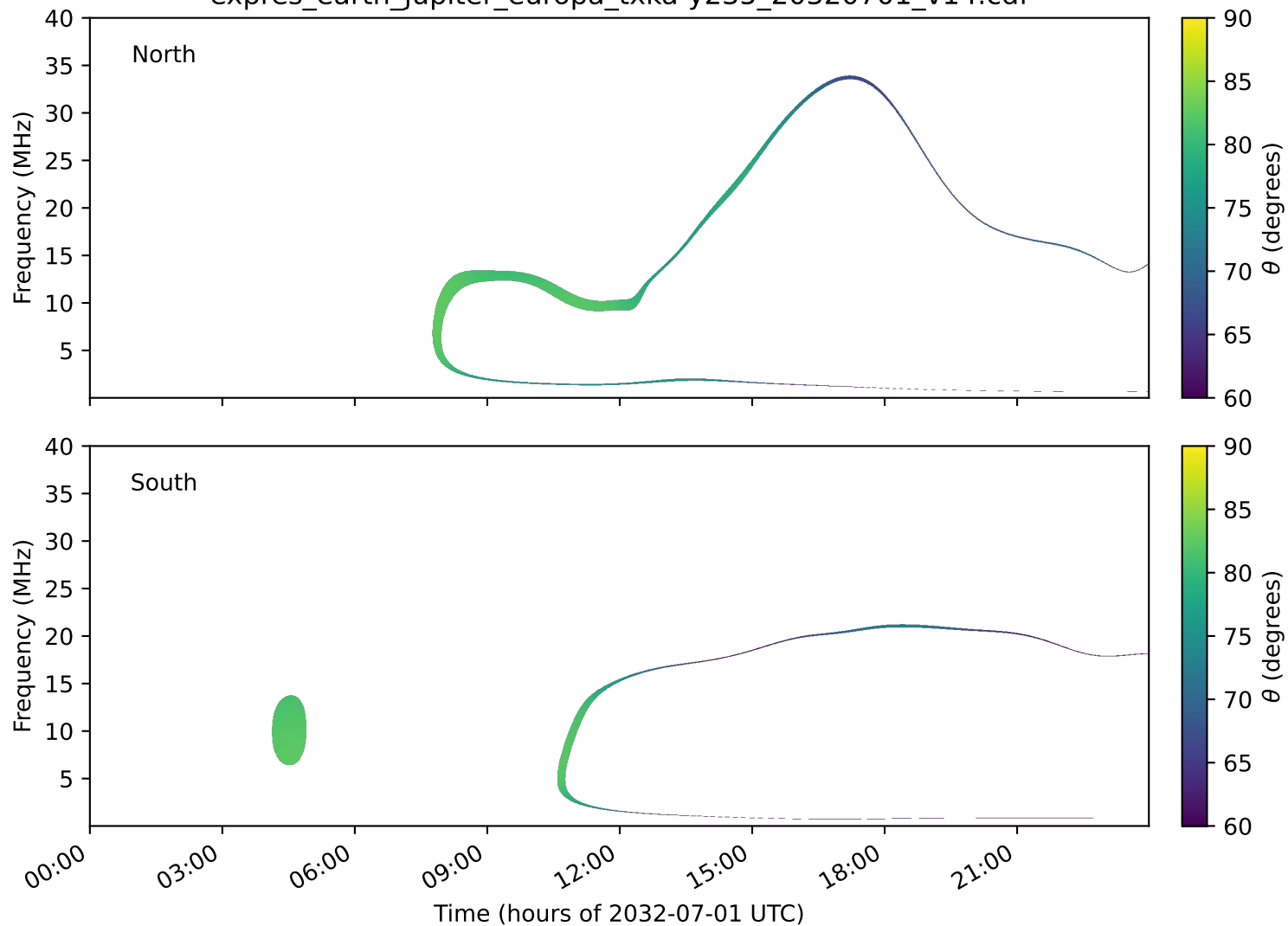
expres_earth_jupiter_europa_txka-y235_20320701_v14.cdf
